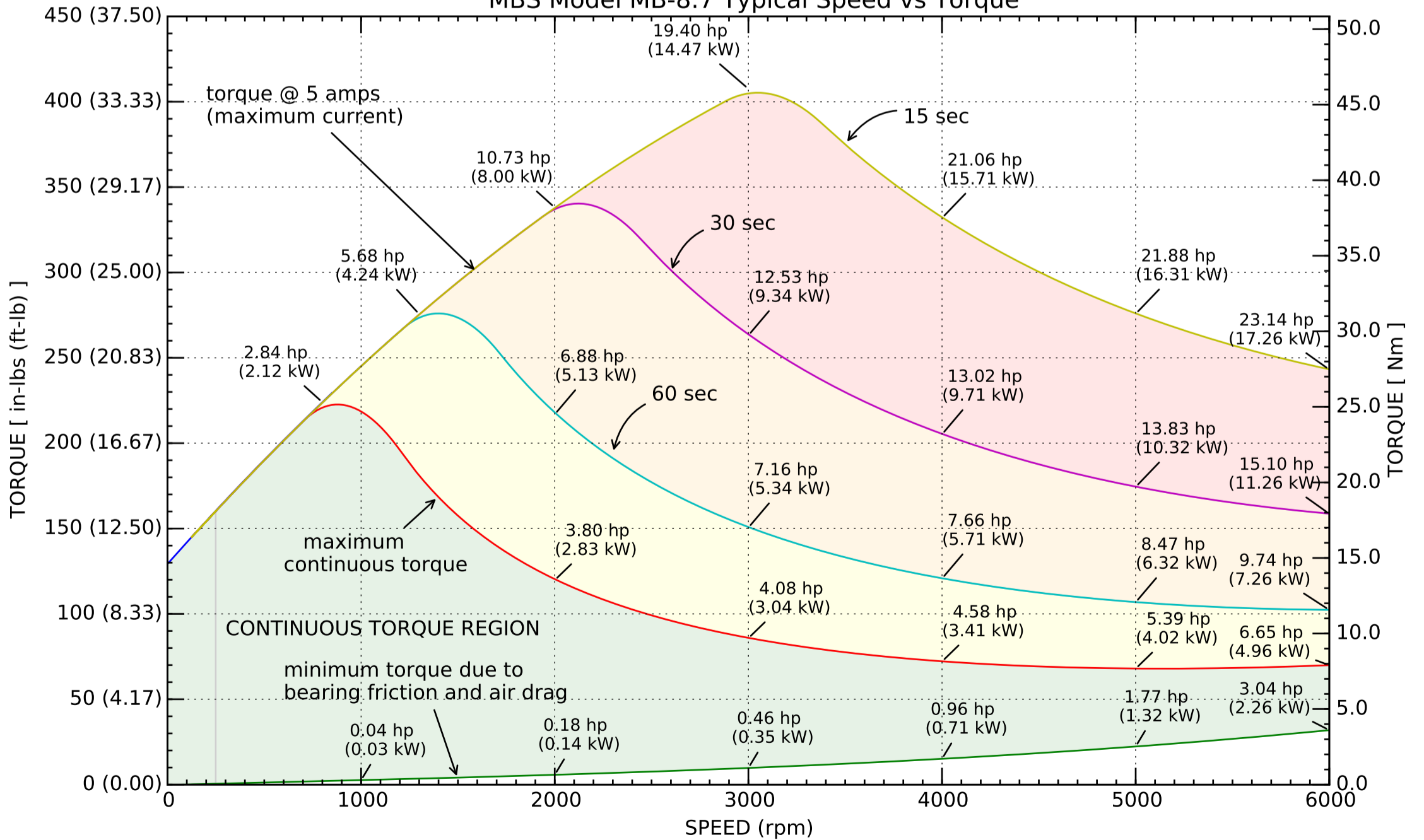
MBS Model MB-8.7 Typical Speed vs Torque
